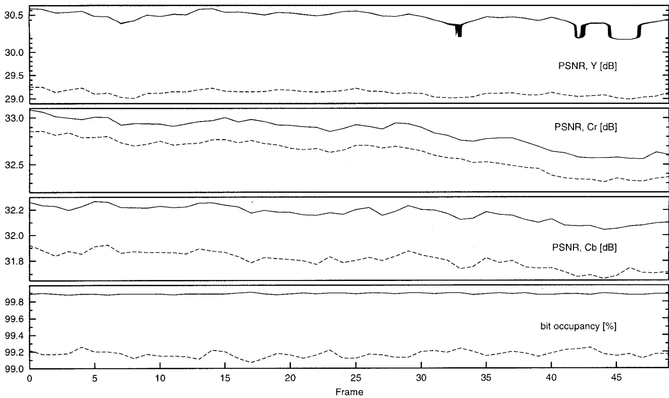
Fig. 12. Results for 50 frames in Mobile Calendar sequence. The solid lines represent the results of the proposed method and the dotted lines represent those of the conventional method.
