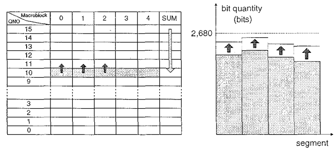
Fig. 3. The procedure and expected result of adjusting QNO
