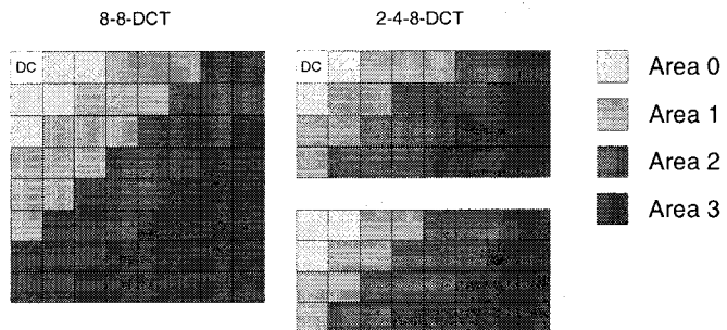
Fig. 2. The structures of DCT blocks
