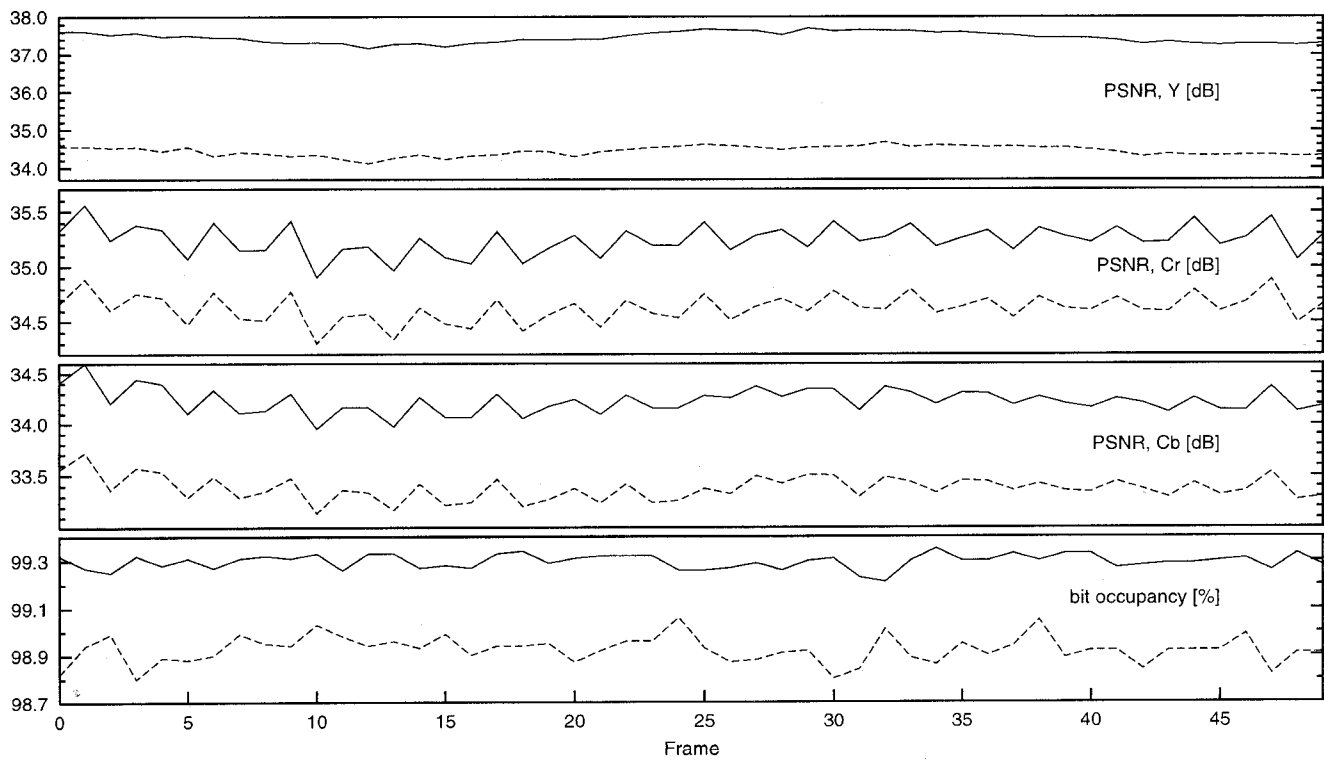
Fig. 13. Results for 50 frames in Popple sequence. The solid lines represent the results of the proposed method and the dotted lines represent those of the conventional method.
