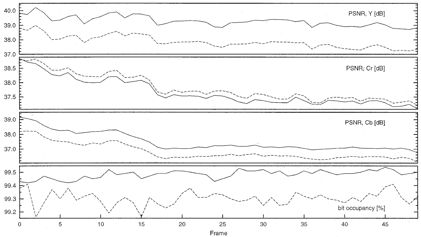
Fig. 11. Results for 50 frames in Football sequence. The solid lines represent the results of the proposed method and the dotted lines represent those of the conventional method.
