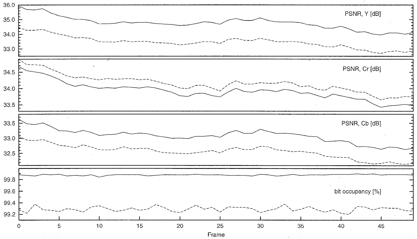
Fig. 10. Results for 50 frames in Flower Garden sequence. The solid lines represent the results of the proposed method and the dotted lines represent those of the conventional method.
