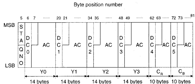
Fig. 1. The structure of a compressed macroblock.
