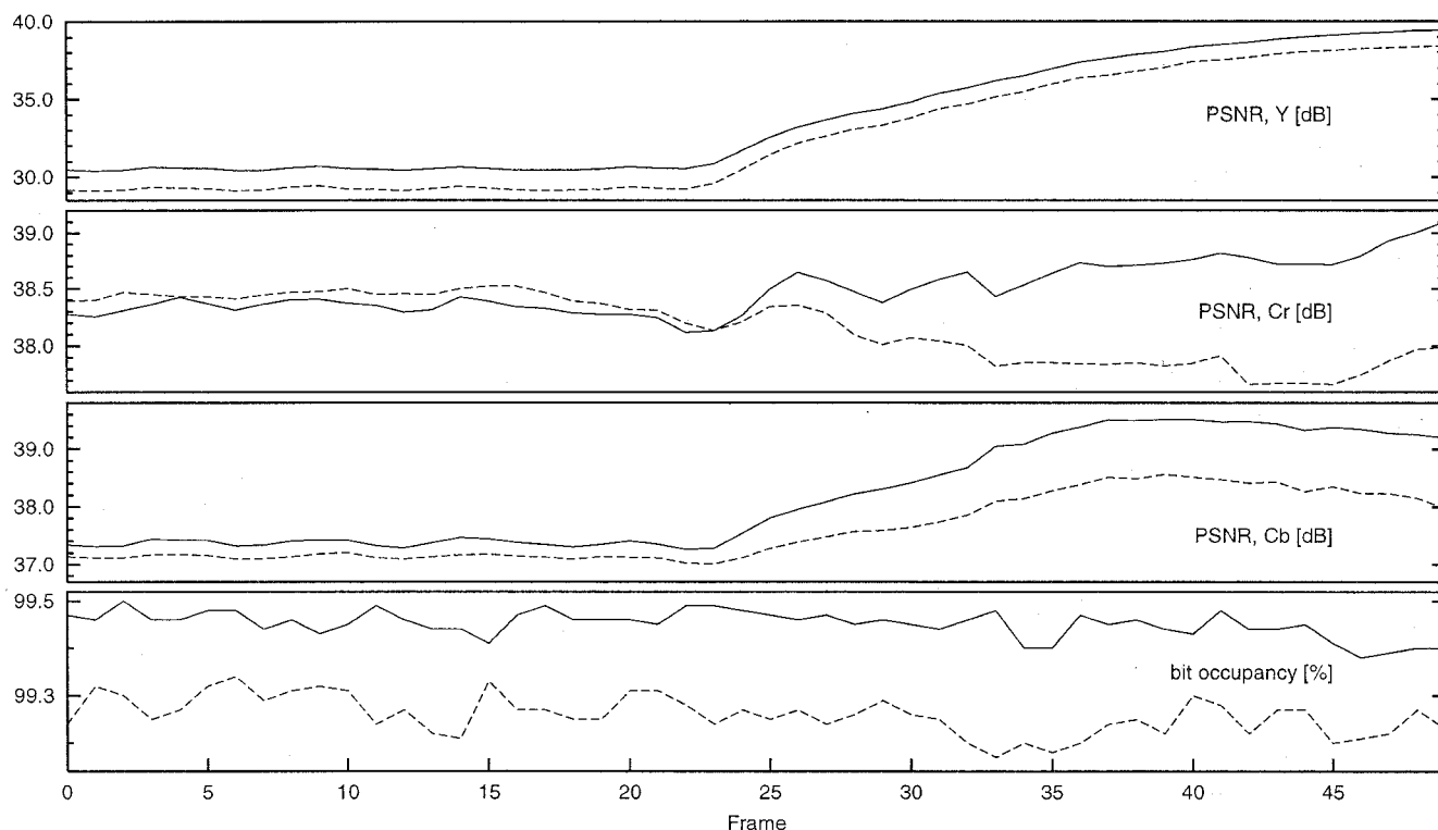
Fig. 14. Results for 50 frames in Table Tennis sequence. The solid lines represent the results of the proposed method and the dotted lines represent those of the conventional method.
