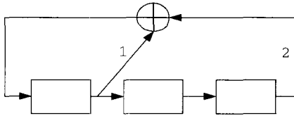
Fig. 1. The LFSR generating S and T 's of Example 7.
